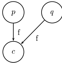
Figure 9: Non-inlinable field
