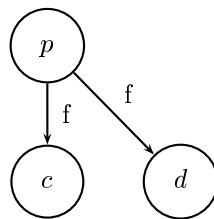
Figure 7: Unique-store field
