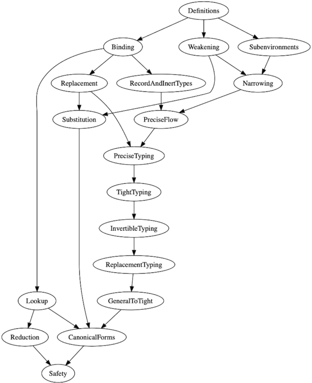
Fig. 16. Dependency between Coq proof files
