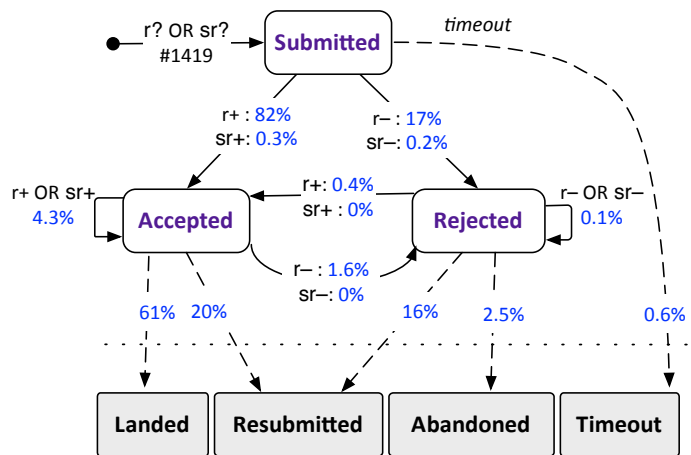
Fig. 2. Mozilla Firefox's patch lifecycle.
