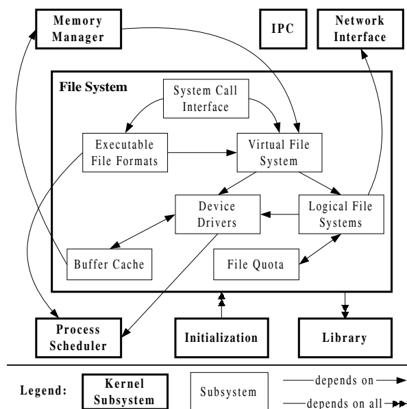
Figure 2: File System Conceptual Architecture
