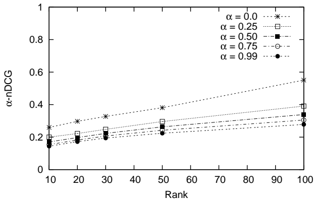
Figure 2: \alpha -nDCG for reversed ideal gain.
