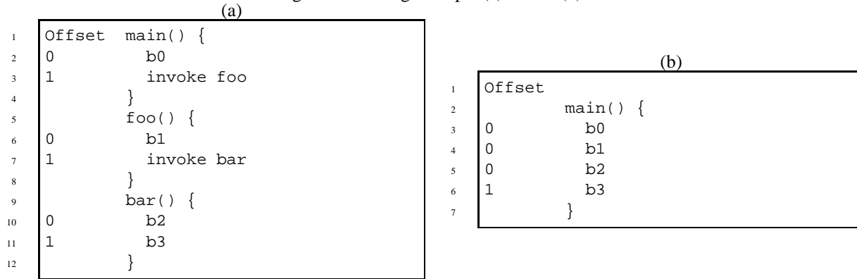
Figure 8: Inlining example (a) before (b) after
